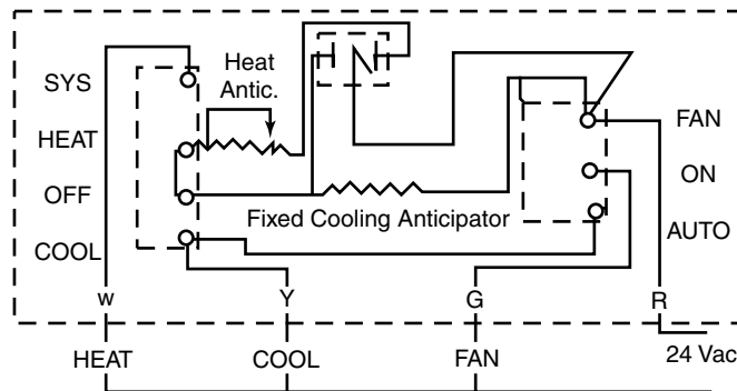
Figure-2 Typical Application for Heating/Cooling Thermostat 31-103 (System: Heat-Off-Cool; Fan: On-Auto).
