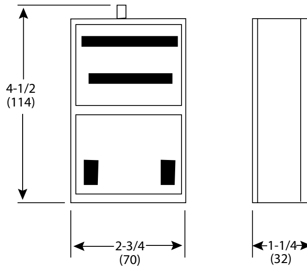
Figure-4 31-102 and 31-103 Dimensions.
