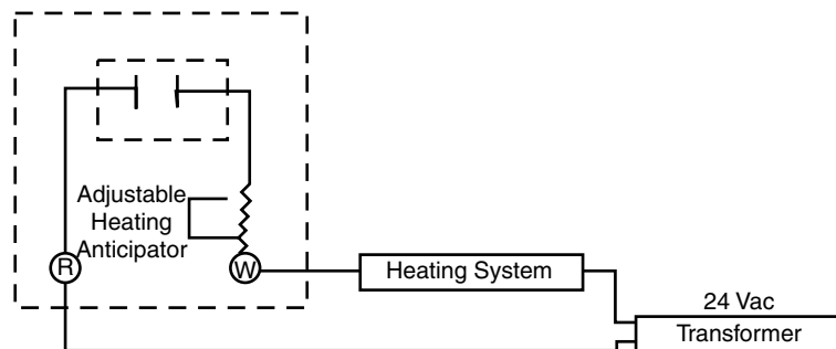
Figure-1 Typical Application for Heating Thermostat 31-102 (No System or Fan Switches).
