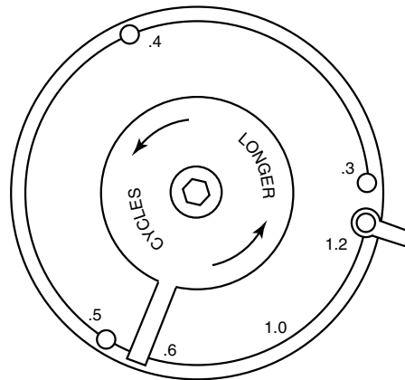
Figure-3 Heat Anticipator.
