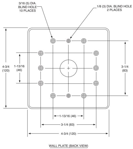
Figure-12 Adapter Plate.
