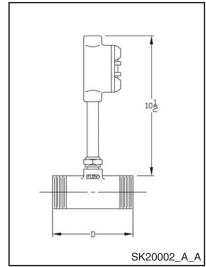
Figure 7 SCH40 MNPT
