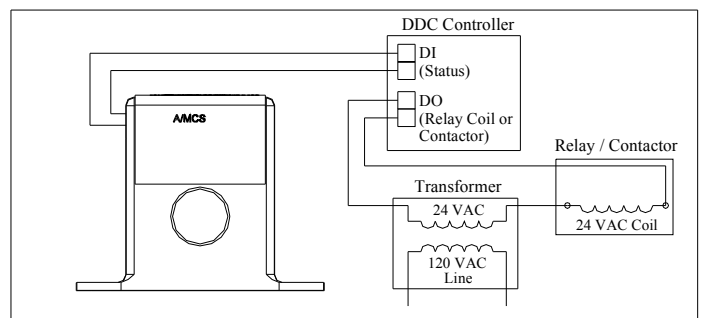
Figure 6: Analog Circuit
