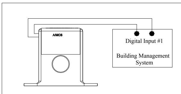
Figure 5: Digital Circuit
